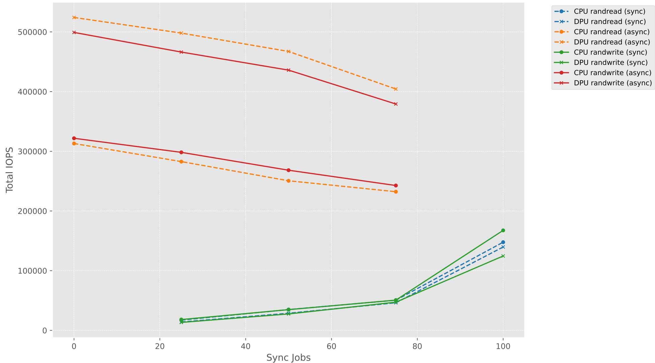
IOPS vs Sync Jobs (mixed) - RAND (CPU vs DPU)
